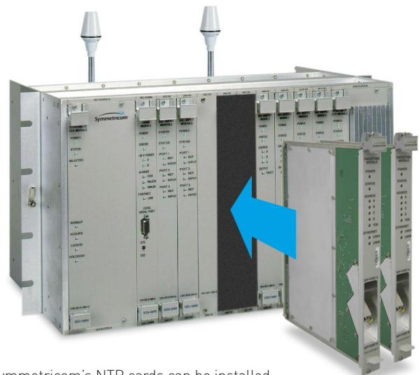
FIG 2: Symmetricom's NTP cards can be installed as single servers or redundant pairs in any available master or expansion shelf output slots.
